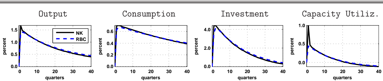
Figure 3: Response to a TFP Shock: Output and Components
