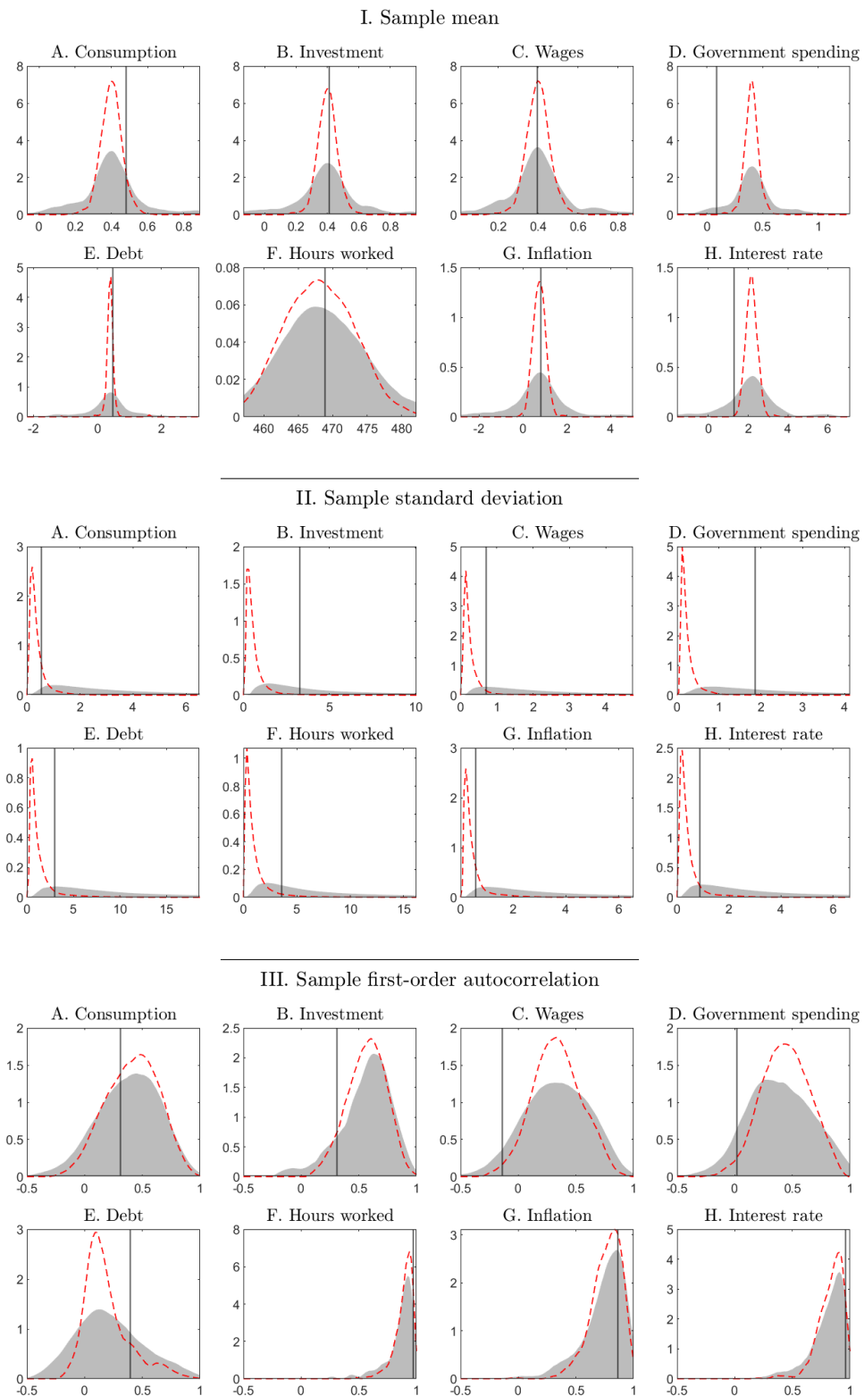
Figure 1: Distributions of simulated selected quantities obtained by sampling the prior, and then the outcomes given drawings from the prior. Notes: Each panel compares the resulting densities under Gaussian shocks with constant volatility (red dashed line) with that under Student- t shocks with stochastic volatility (shaded area). Vertical lines denote the real data counterparts.
