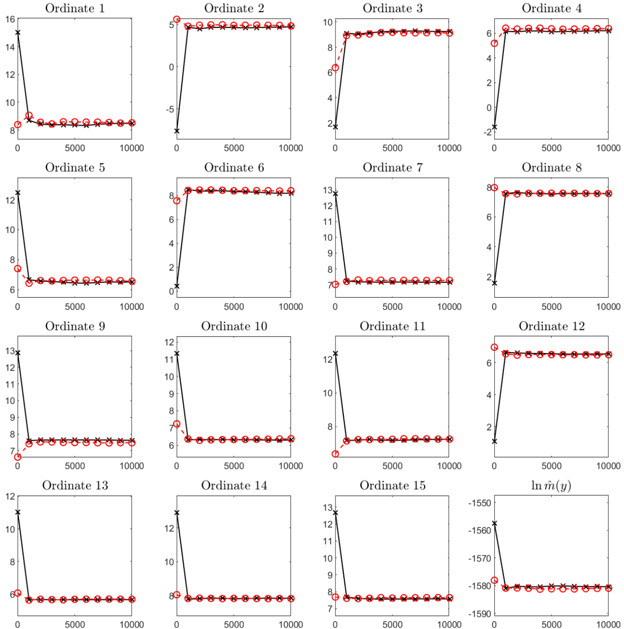
Figure 4: Recursive posterior ordinates and marginal likelihood. Notes: Ordinates 1–7 (8–15) correspond to structural (volatility) parameters. The last panel depicts the estimated marginal likelihood. Black solid lines (with cross marker) correspond to the benchmark setting ( p = 0.7 , \omega = 0.5 ). All estimates are in logarithm scale.
