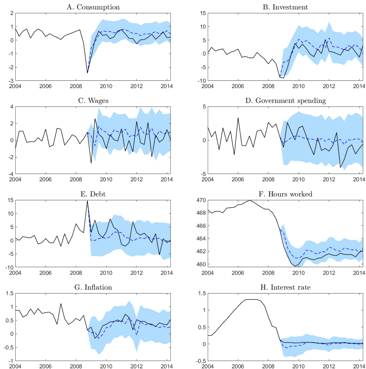
Figure 5: DSGE-model forecast of each observable. Notes: Each panel compares the one-quarter-ahead posterior forecast of regime M with real data (black solid lines). Blue dashed lines denote median forecasts, while blue shaded areas delineate 90% highest predictive density bands.
